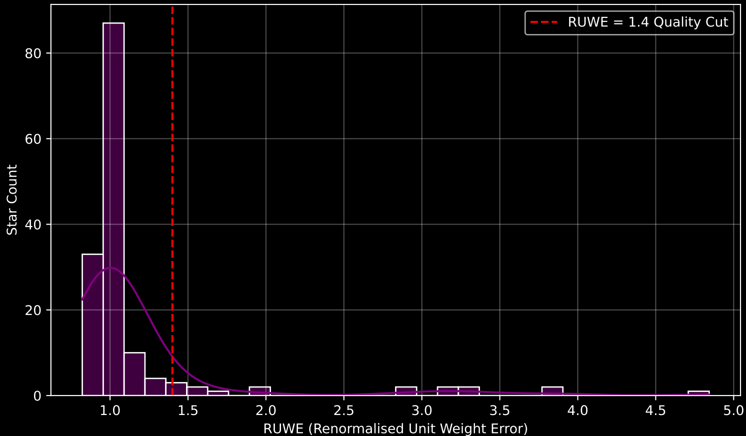
GAPOGEE DR17 Field [045+36_MGA] RUWE Distribution (n= 151)
