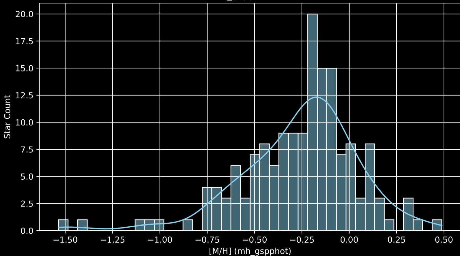
APOGEE DR17 Field: [045+36_MGA [M/H] (mh_gspphot) (n= 159)
