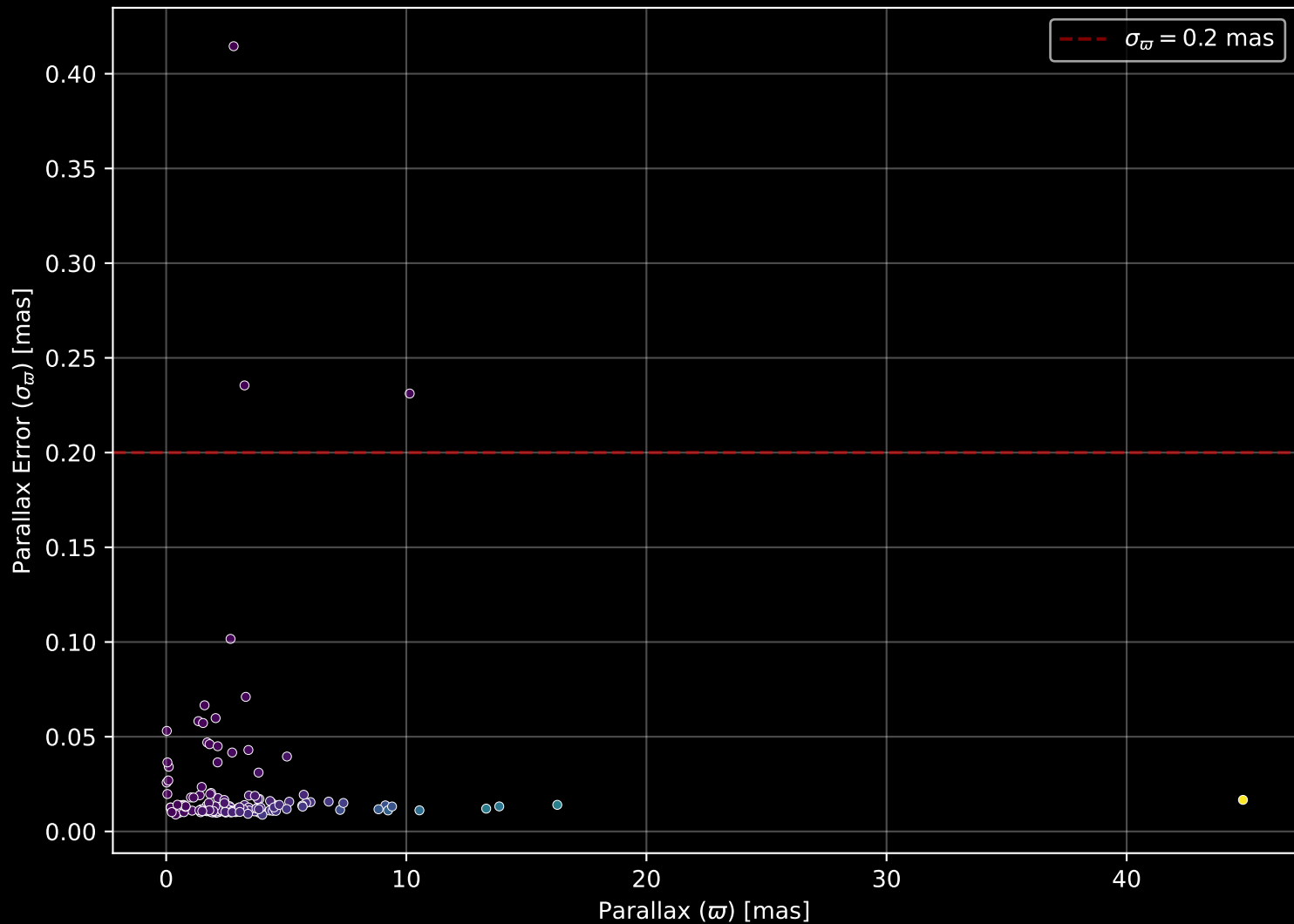
APOGEE DR17 Field: [045+36_MGA] Parallax Quality (n= 159)
