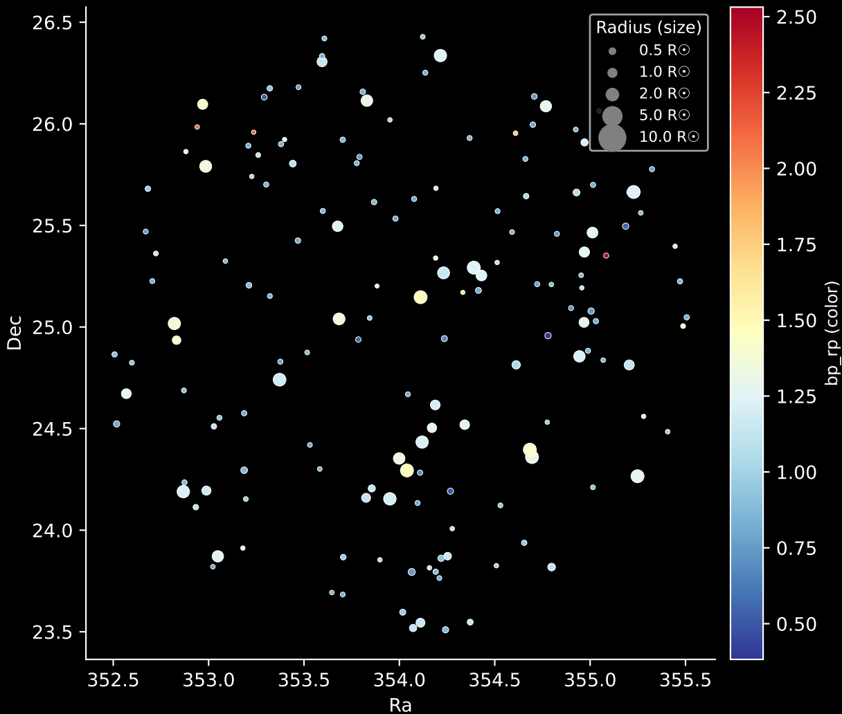
APOGEE DR17 Field: [045+36_MGA] Stars: 159
