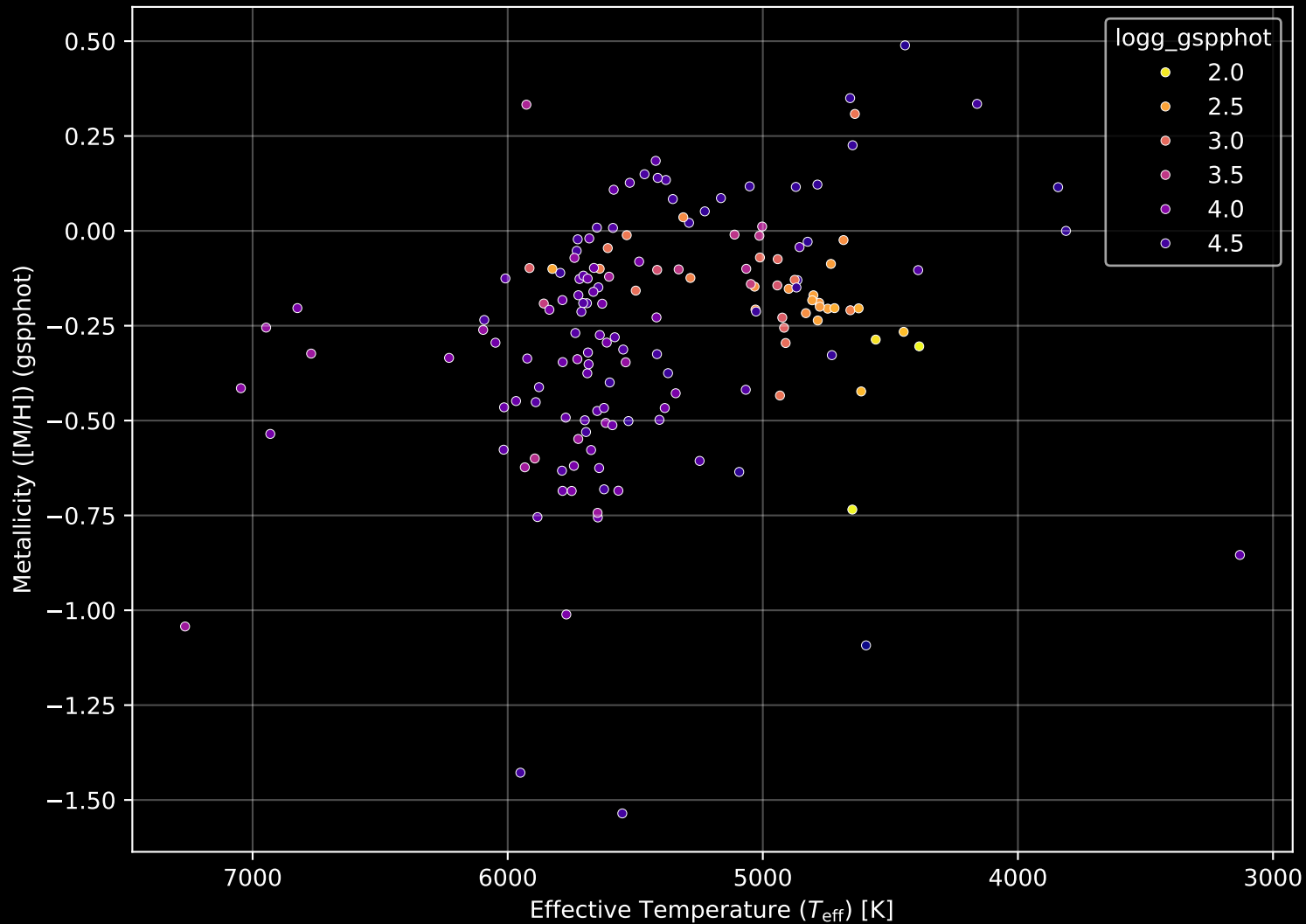
APOGEE DR17 Field: [045+36_MGA] Stellar Population Parameters (n= 159)
