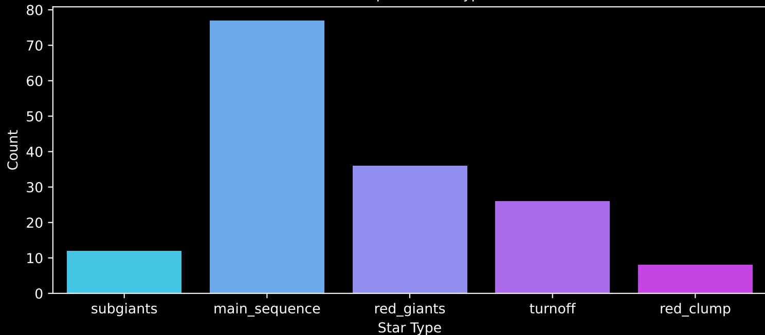
APOGEE DR17 Field: [045+36_MGA] Count plot of Star Type
