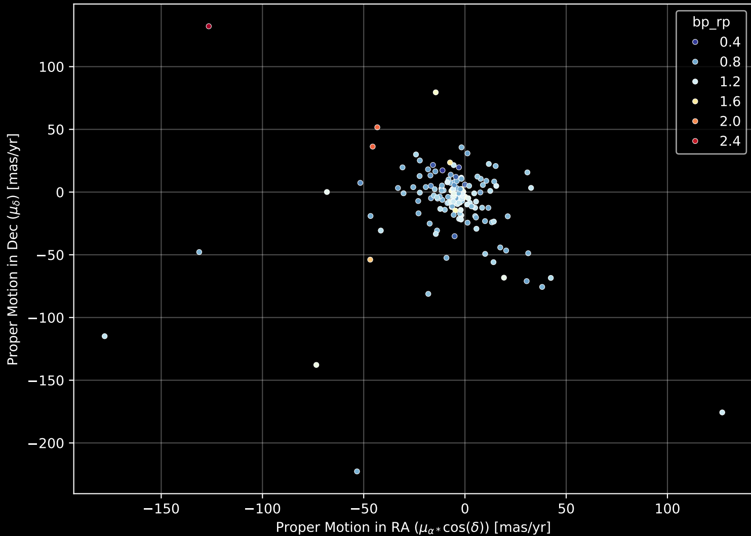
APOGEE DR17 Field: [045+36_MGA] Proper Motion Diagram (n= 159)
